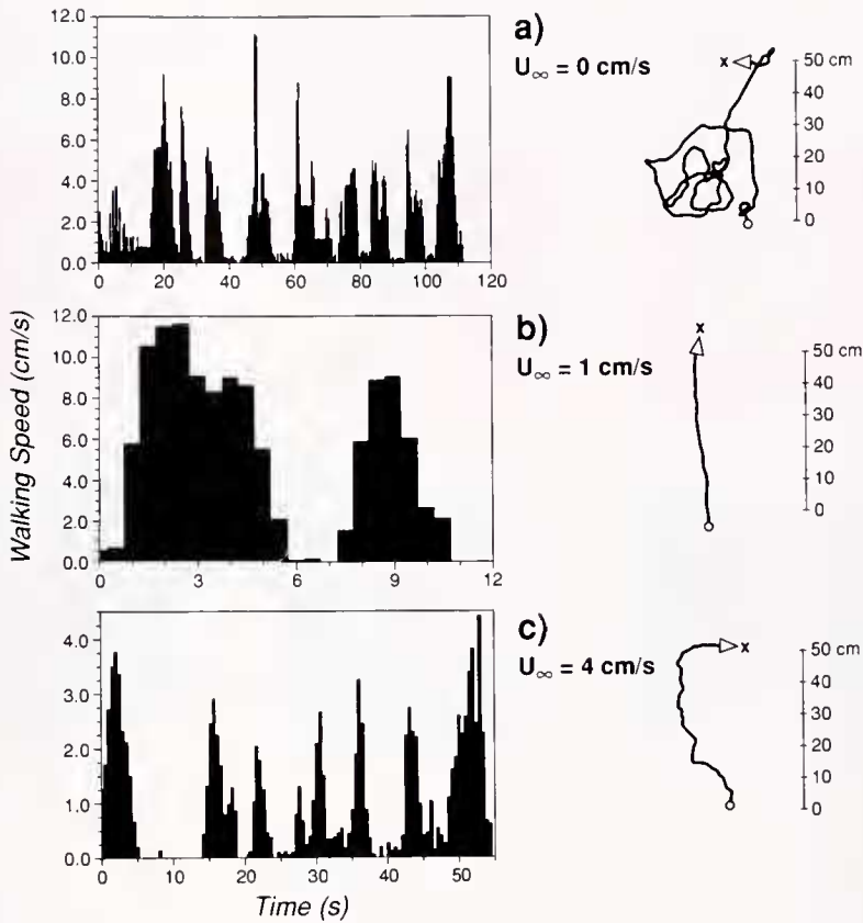
Figure 4. Using computer-assisted video motion analysis, traces to the right are paths walked by blue crabs as they searched for clams in a 10-m-long raceway flume at flow speeds of 0, 1, and 4 cm/s (top to bottom). Each 'O' marks the location where a search began, and each 'X' indicates the ultimate site of clam capture. Graphs to the left are histograms of walking speed versus time plotted for each path displayed to the right. The most efficient paths were those walked by crabs in 1 cm/s flow. In each case, intermittent walking and stopping characterized a search. The "stop interval" was defined as the time when crabs reset their attack angle ( i.e. , turned) before moving on.
